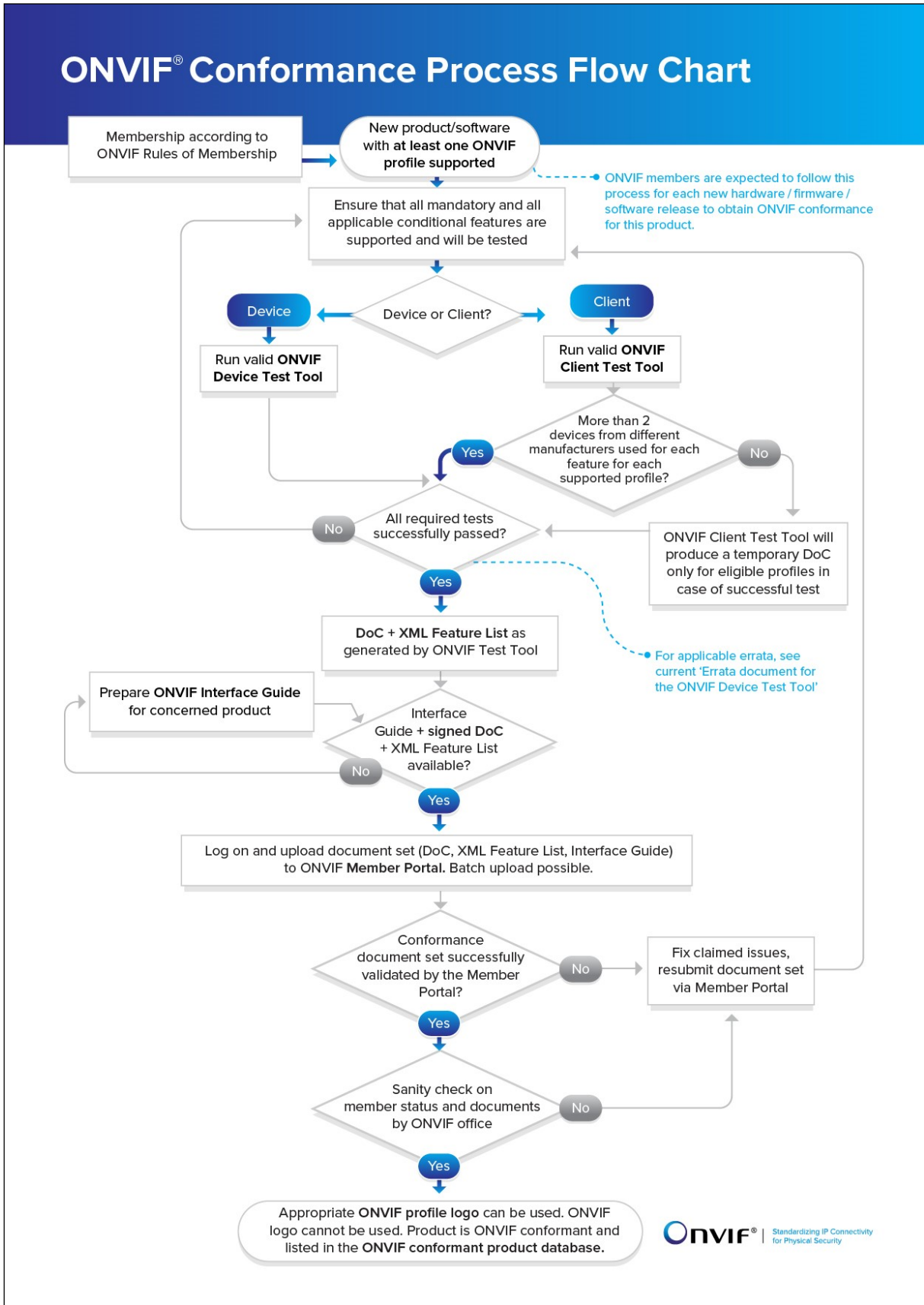
Fig. 1: ONVIF Conformance Process flow chart
