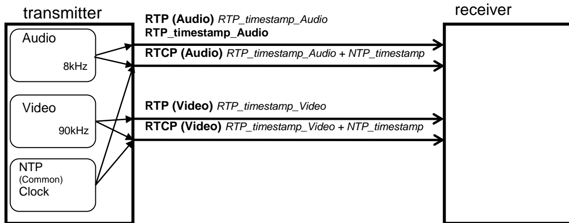
Figure 5: Media Synchronization
