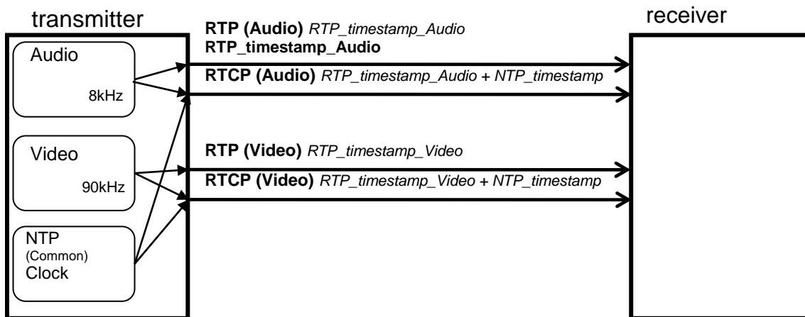
Figure 5: Media Synchronization
