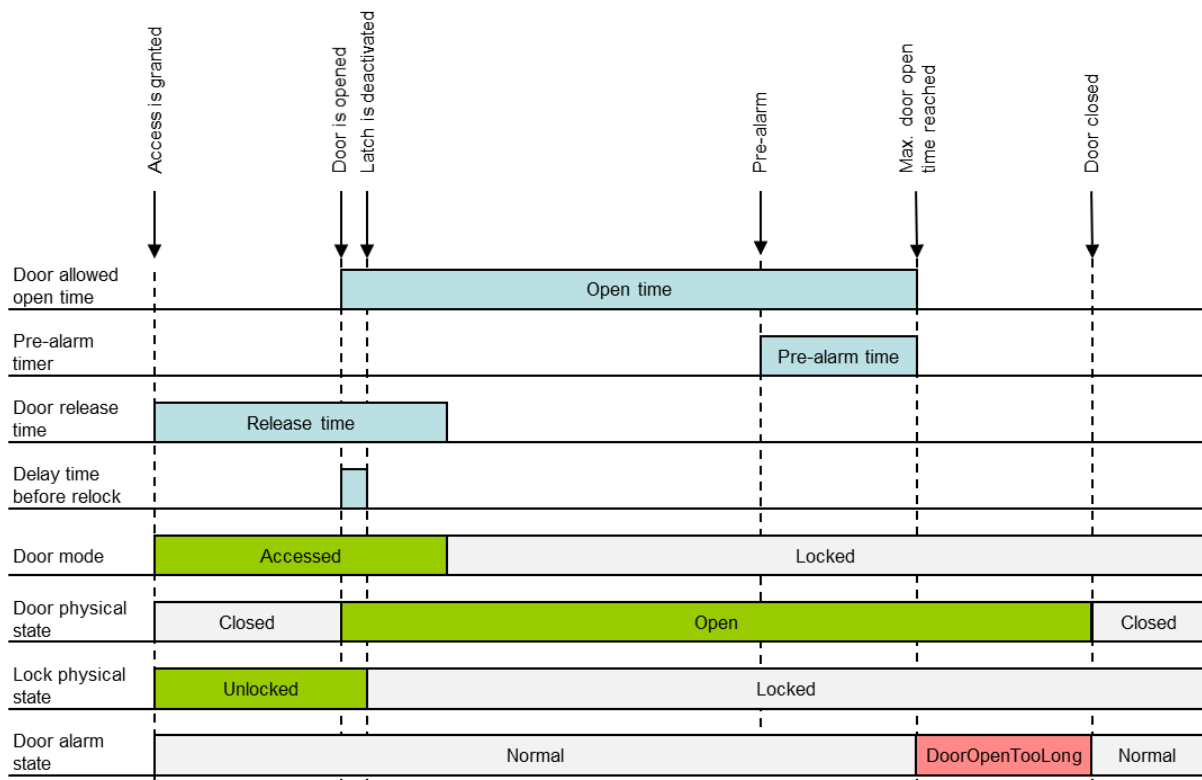
Figure 2: Door timings
