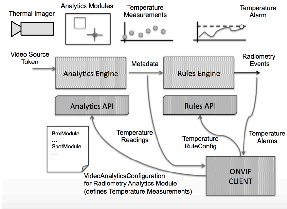
Figure 4 Radiometry Analytics Modules, Rules, Metadata and Events
