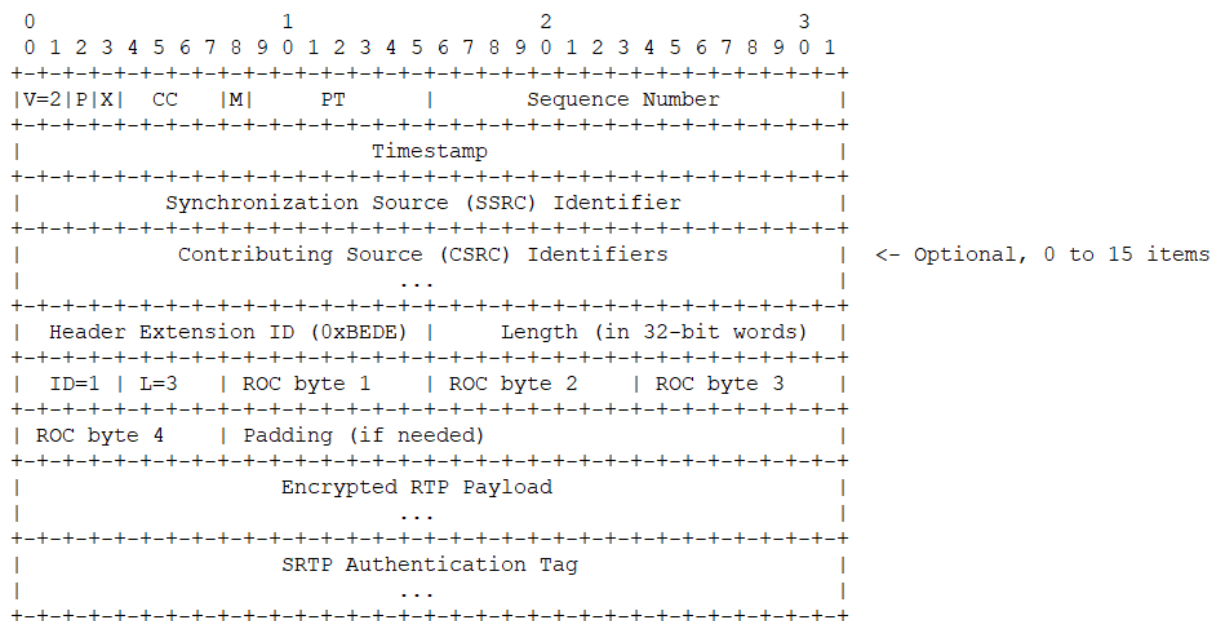
Figure 12: Diagram of SRTP packet format with ROC extension
