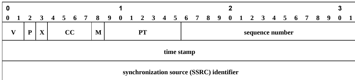
Figure 2: RTP header
