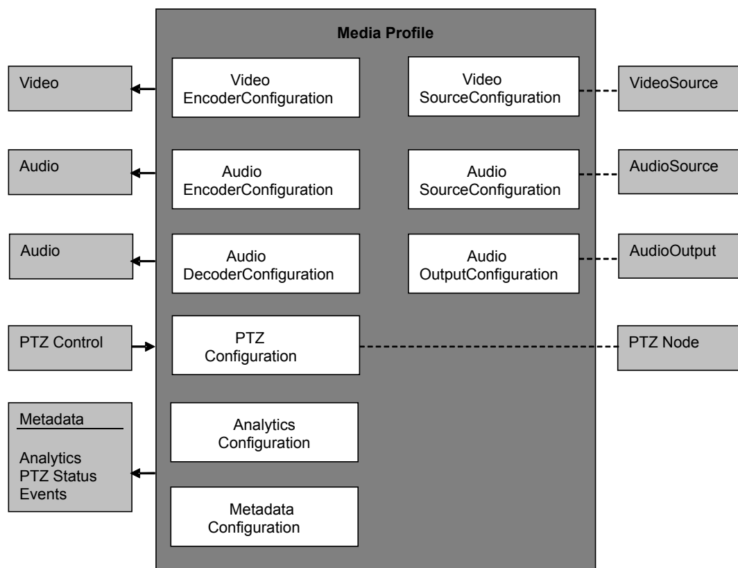
Figure 2: Complete profile configuration
