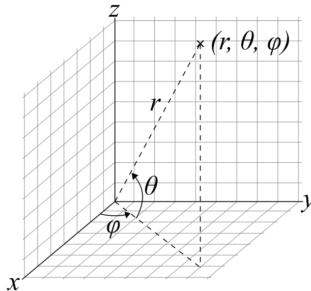
Figure 3: Spherical coordinates
