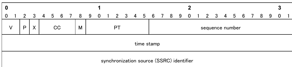
Figure 2: RTP header
