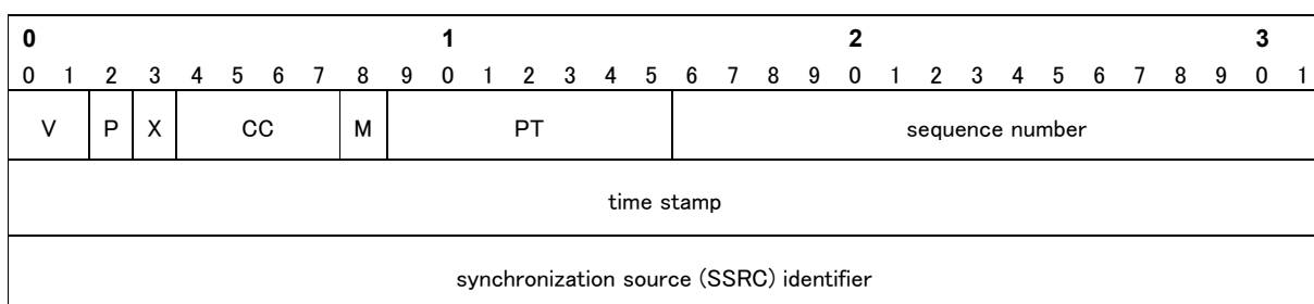
Figure 2: RTP header
