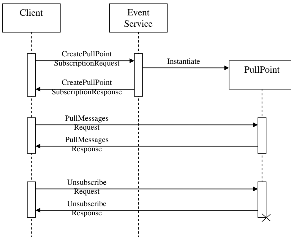
Figure 9: Sequence diagram for the Real-time Pull-Point Notification Interface.
