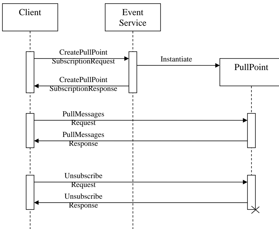
Figure 3: Sequence diagram for the Real-time Pull-Point Notification Interface.
